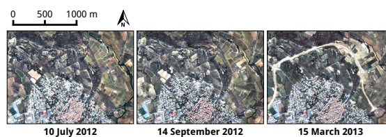
Figure 3: Visible color composite of the three Pleiades images showing the construction of a bypass north of Villeveyrac (France).
