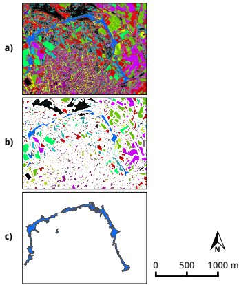
Figure 4: Clustering, segmentation and vector output from the Pleiades time series processing around the Villeveyrac area.
