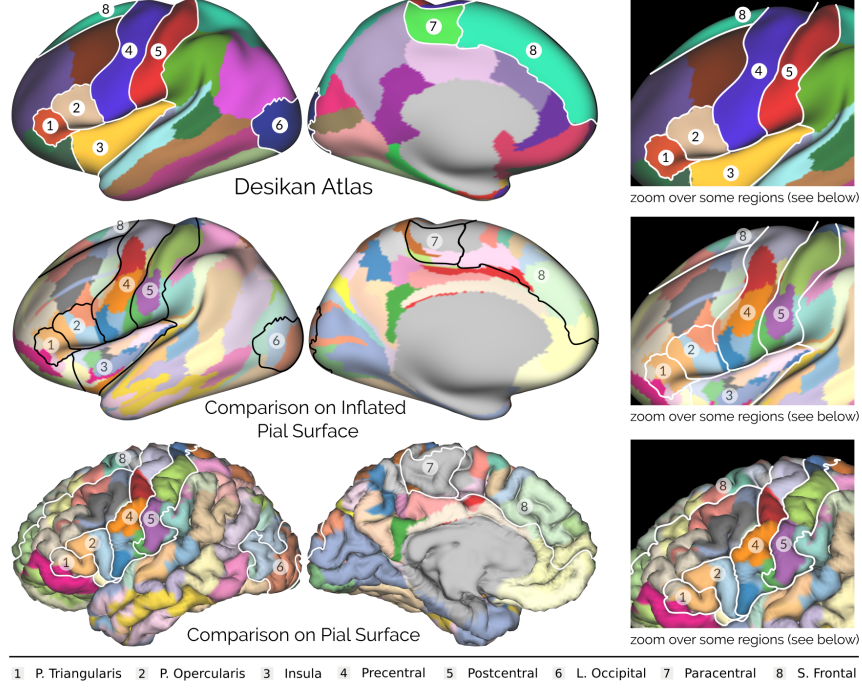
Fig. 5: Relation between our pure extrinsic parcellation and the anatomical atlas of Desikan [5]. Some regions from Desikan projected over a parcellation with less than 150 parcels. Motor and Sensitive cortex appears to be found.
