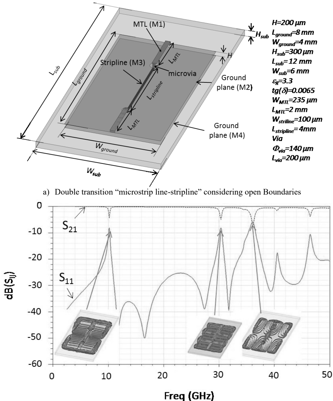
b) EM simulating S parameters results Fig. 2: Double microstrip to stripline transition (a) and S parameter measurement results (b) with open boundary conditions
