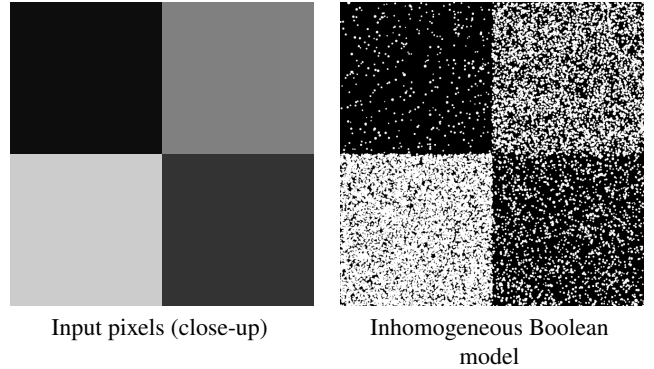
Figure 4: Illustration of inhomogeneous Boolean model. The local intensity \lambda(y) of the inhomogeneous Boolean model is chosen to respect the input pixel gray-levels.
