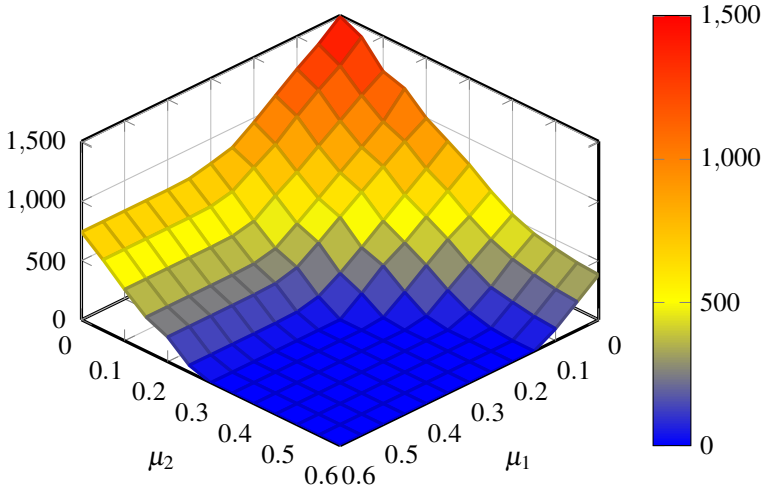
Response surface of reaction force
