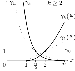
FIGURE 1. The functions x \mapsto \gamma_k(x) and q \mapsto \gamma_k(n/q) are both convex, and such that \gamma_k(n/2) = 1 .
