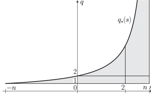
FIGURE 2. The optimal constant C_{q,s} in (7) is independent of q and determined for any given s by the critical case q = q_*(s) : the Hardy-Littlewood-Sobolev inequality (1) if s \in (-n, 0) and the Sobolev inequality (5) if s \in (0, n) . The case s = 0 is covered by Corollary 11, while q = 2 corresponds to the fractional logarithmic Sobolev inequality (18) if s = 0 and the subcritical fractional logarithmic Sobolev inequality by Corollary 4 if s \in (0, n] .
