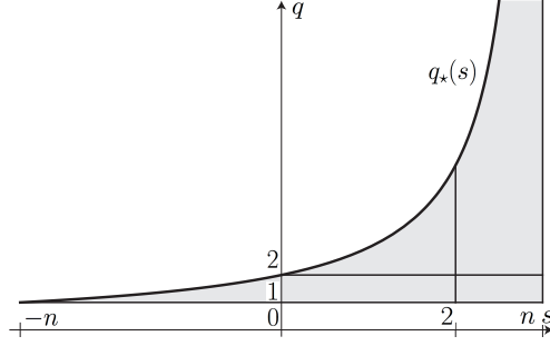
FIGURE 2. The optimal constant C_{q,s} in (7) is independent of q and determined for any given s by the critical case q = q_*(s) : the Hardy-Littlewood-Sobolev inequality (1) if s \in (-n, 0) and the Sobolev inequality (5) if s \in (0, n) . The case s = 0 is covered by Corollary 11, while q = 2 corresponds to the fractional logarithmic Sobolev inequality (18) if s = 0 and the subcritical fractional logarithmic Sobolev inequality by Corollary 4 if s \in (0, n] .
