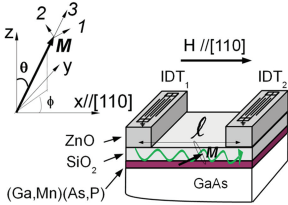
FIG. 1. (Color online) Structure of the sample (not to scale). 50 nm ferromagnetic epilayer, 70 nm \text{SiO}_2 buffer, and 250 nm piezoelectric ZnO. The IDTs have an aperture of 1 mm and are separated by 2 mm, but the effective length of the delay line is taken center to center of the IDTs, i.e., l = 2.3 mm. Upper left: Definition of the (x, y, z) and (1, 2, 3) reference frames.
