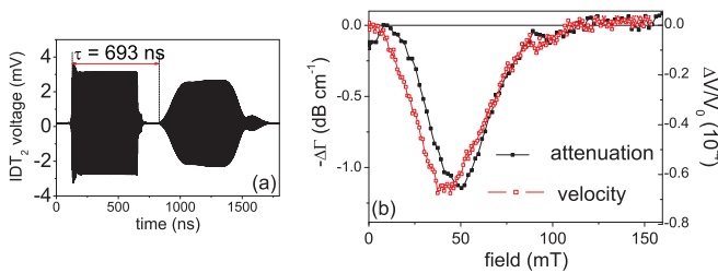
FIG. 2. (Color online) (a) Receiving IDT signal: The electromagnetic field radiated by the emitter is shortly followed by the transmitted surface acoustic wave. T = 120 K, 549 MHz. (b) Acoustic attenuation changes and relative velocity variations at T = 80 K. The opposite of \Delta\Gamma has been plotted in order to highlight the different resonant field from the velocity variations.
