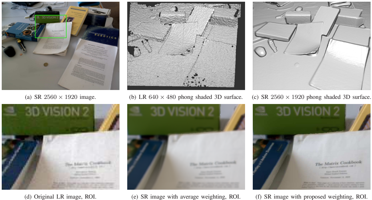
Fig. 4. (a) Super-resolved image of dimensions 2560 \times 1920 pixels. (b) Phong shading of the original 3D surface before optimisation. (c) Phong shading of the SR 3D surface after optimisation. (d) Region of interest of the original image. (e) Region of interest of the SR image with the average weighting after optimisation. (f) Region of interest of the SR image with the proposed weighting after optimisation. It can be seen that the SR SLAM algorithm greatly improves depth measurements as well as intensity measurements. Compared to standard averaging (e) the proposed approach considers the pose of the camera in the weighting function and produces better resolved results.
