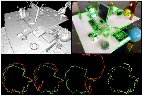
Figure 3: On the left Kinfu result for freiburg_desk2 sequence using 3x3x3, 5x5x5 and 8x8x8 meter voxel volume. Kinfu gains lower drift due to structural optimization, but planar surfaces cause tracking failures. 3x3x3 volume does not contain floor and therefore Kinfu works well. Limited operating volume is a problem for practical use in the studio. On the right, our dense tracking drift illustrated when a fixed keyframes are not used. Problems with planar surfaces or limited operating volume do not exist. Green dots reveal the selected points for given RGB-D measurement.
