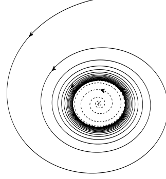
Fig. 1. Trajectories of the Andronov-Hopf oscillator on the complex plane. If \mu_R > 0 the origin is unstable but all trajectories tend to a stable limit-cycle of radius r = \sqrt{\mu_R/\nu_R}
