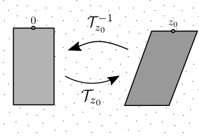
FIGURE 2. The transformation leaving the equation invariant. On the left, a straight cylinder centered at the origin. On the right a slanted cylinder centered at z_0 .
