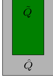
FIGURE 3. The cylinders \hat{Q} and \tilde{Q}
