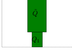
FIGURE 5. Geometric setting of the propagation Lemma 9.1.
