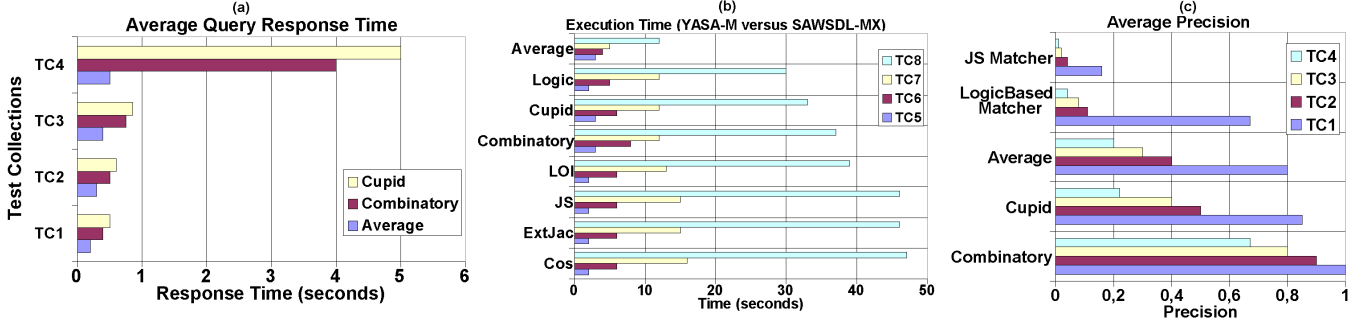
Fig. 6. Evaluations and Experiments.
