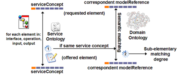
Fig. 3. Elementary / Semantic Matching.
