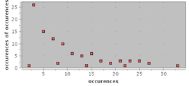
Fig. 5. Profile Curve of the Distribution.
