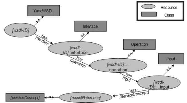
Fig. 2. The Generic RDF Tree ([serviceConcept] is replaced by the name of the service concept of the YASA semantic annotation and [modelReference] by the model reference of the YASA semantic annotation).
