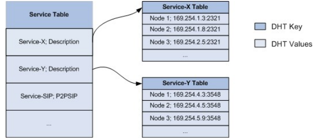
Figure 2. DHT API
