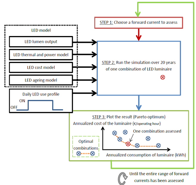
Fig. 2. Flowchart of the LED optimization methodology
