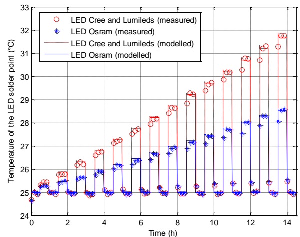
Fig. 9. Evolution of LED solder point temperatures
