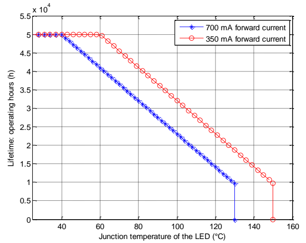
Fig. 10. Simplified lifetime model of an LED [26]
