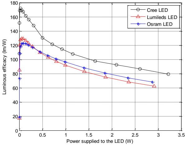
Fig. 4. Luminous efficacy vs. Power for the three tested LEDs
