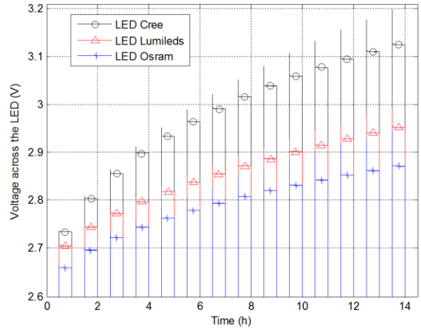
Fig. 8. Voltage across each LED for different forward currents
