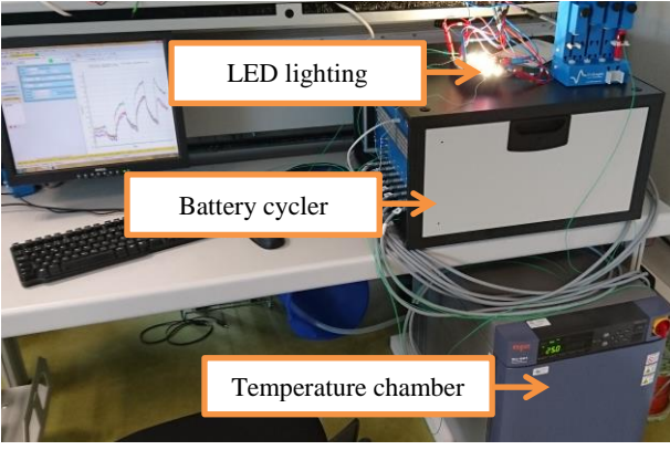
Fig. 3. Experimental setup assessing LEDs
