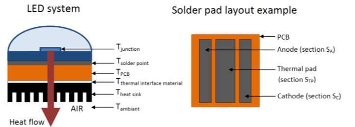
Fig. 6. Thermal variables used to model an LED system
