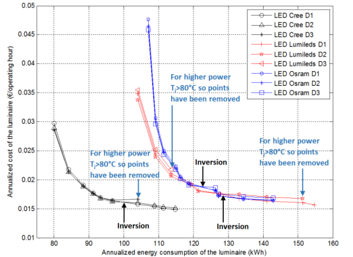
Fig. 11. Annualized cost vs. power of the luminaire
