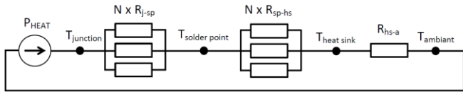
Fig. 7. Thermal model of an LED
