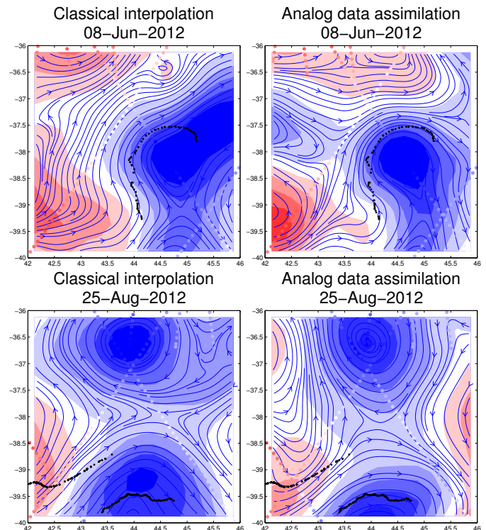
Fig. 2. Interpolation results of along track sea level anomalies using classical spatiotemporal methods and the analog data assimilation. The streamlines represent the corresponding geostrophic currents. Along track observations and drifting buoys trajectories correspond to \pm 2 days of data centered on June 8 th 2012 and August 25 th 2012 in the Agulhas return current.
