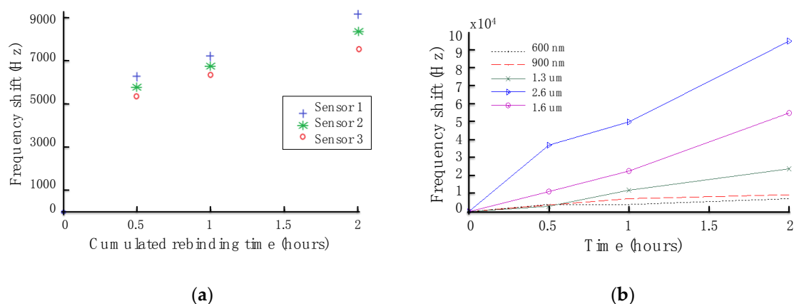
Figure 4. Frequency shift (absolute value) of (a) three sensors to 25 ppm of: AMP as target compound, vs. the rebinding time (0.5, 1 and 2 h). The sensitive films thickness was 1 \mu\text{m} , the extraction time 3 h; and (b) five sensors to 25 ppm of AMP as target compound, vs. the rebinding time (0.5, 1, and 2 h), with the sensitive film thickness as parameter in the range 0.6 \mu\text{m} –2.6 \mu\text{m} .
