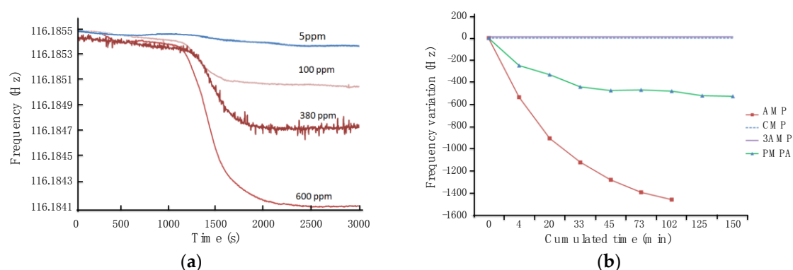
Figure 5. Real-time response of the sensor (a) to different concentrations of AMP as target compound; and (b) to AMP as target compound and specificity to three similar commercial nucleotides, each one at a concentration of 300 ppm.
