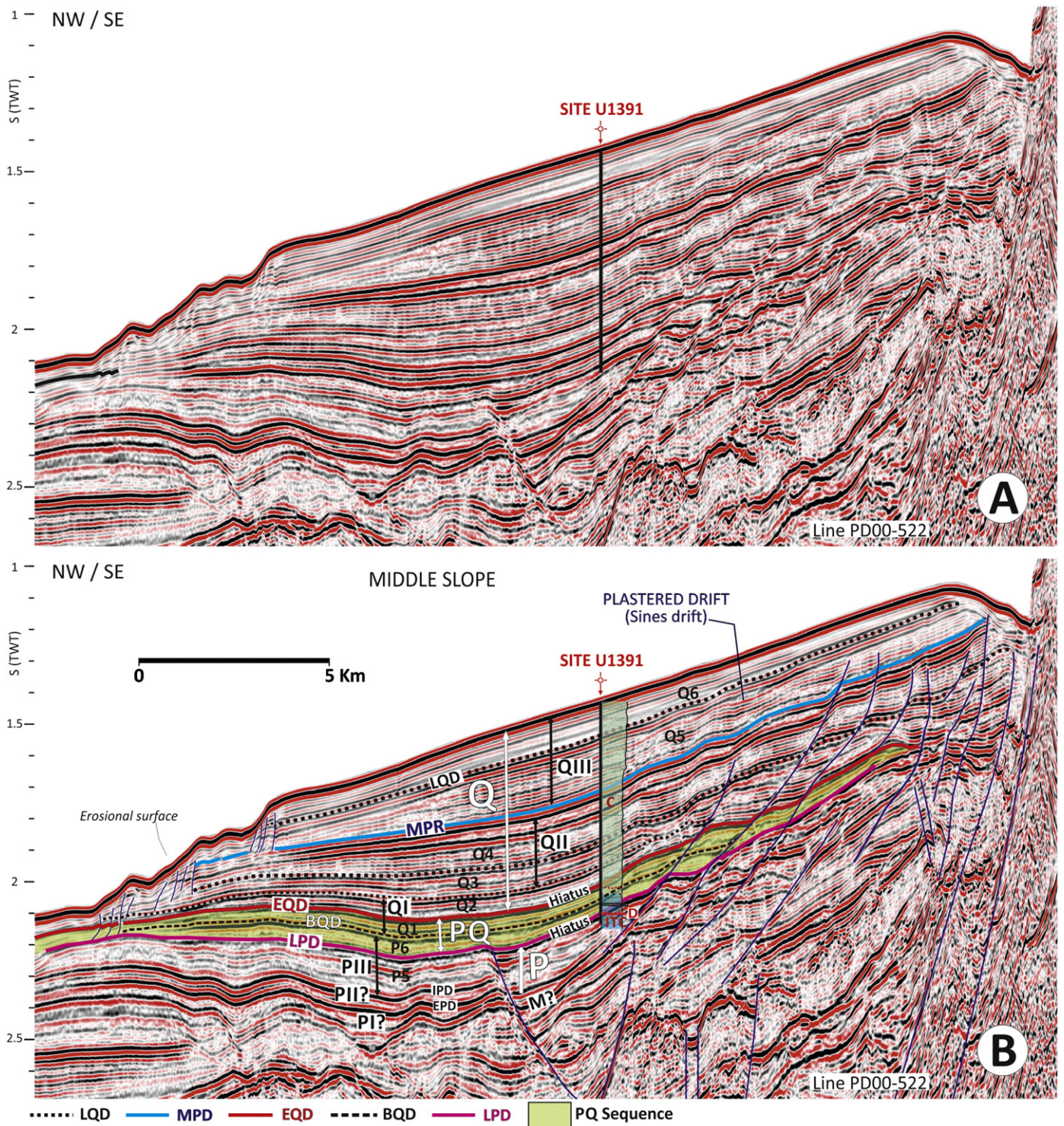
Fig. 14. Seismic profile (line PD00-522) of the Alentejo basin showing the Pliocene to Quaternary sedimentary record at site U1391. Major sequences (P, PQ and Q), units (P1–PIII and Q1–QIII) and subunits (P1–P6 and Q1–Q6), as well as the main discontinuities and hiatus are shown (data courtesy of TGS–NOPEC Geophysical Company ASA). Profile location given Fig. 3. Abbreviations for discontinuities are in Fig. 6. Simplify sedimentary log for U1390 is included (see abbreviations in Fig. 5).
