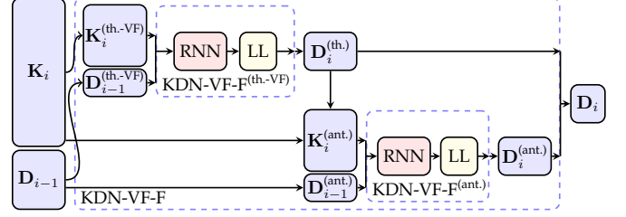
(b) KDN-VF-F: two-stage thumb-virtual finger network.
