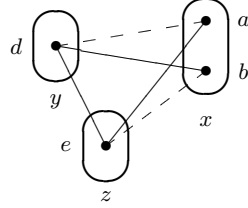
Fig. 1. A broken triangle on two values a, b for a given variable x .
