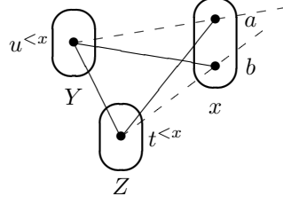
Figure 11: Illustration of a directional general-arity broken triangle.
