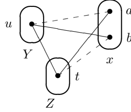
Figure 10: A general-arity broken triangle on values a, b \in \mathcal{D}(x) .
