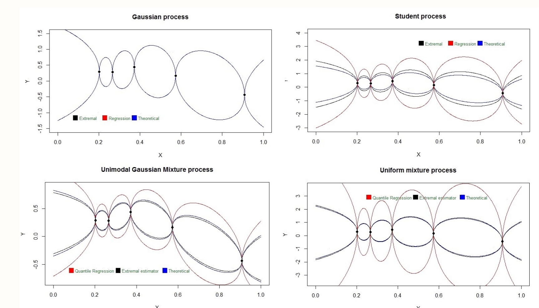
Figure 1: Levels of quantile \alpha = 0.995 and \alpha = 0.005
