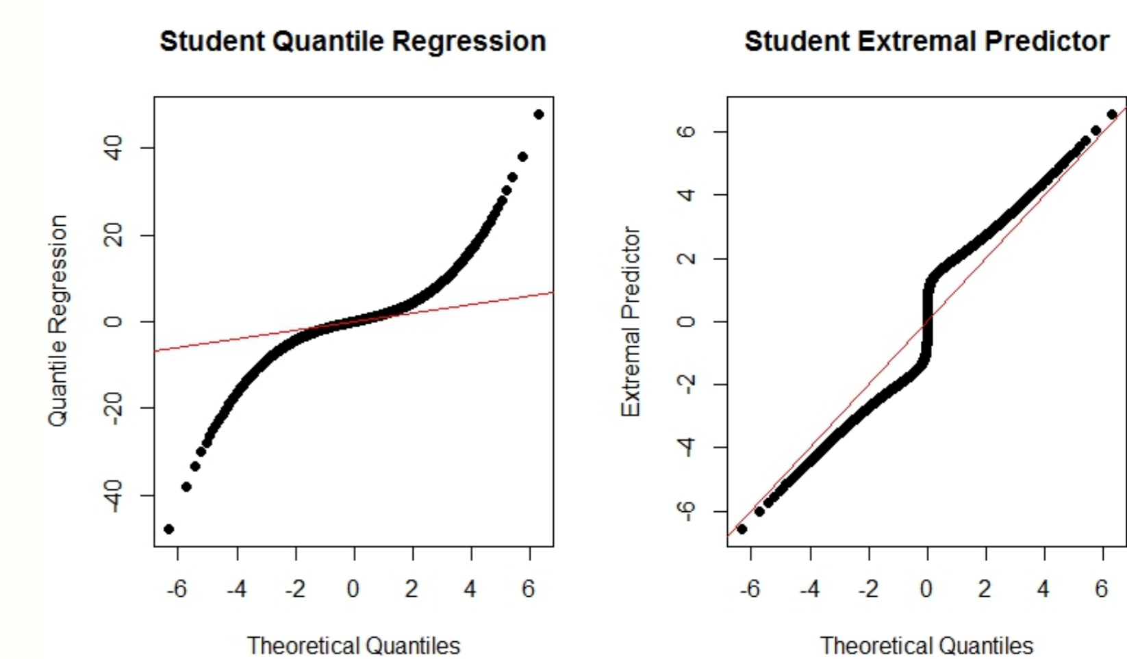
Figure 2: Q-Q plots for Student example
