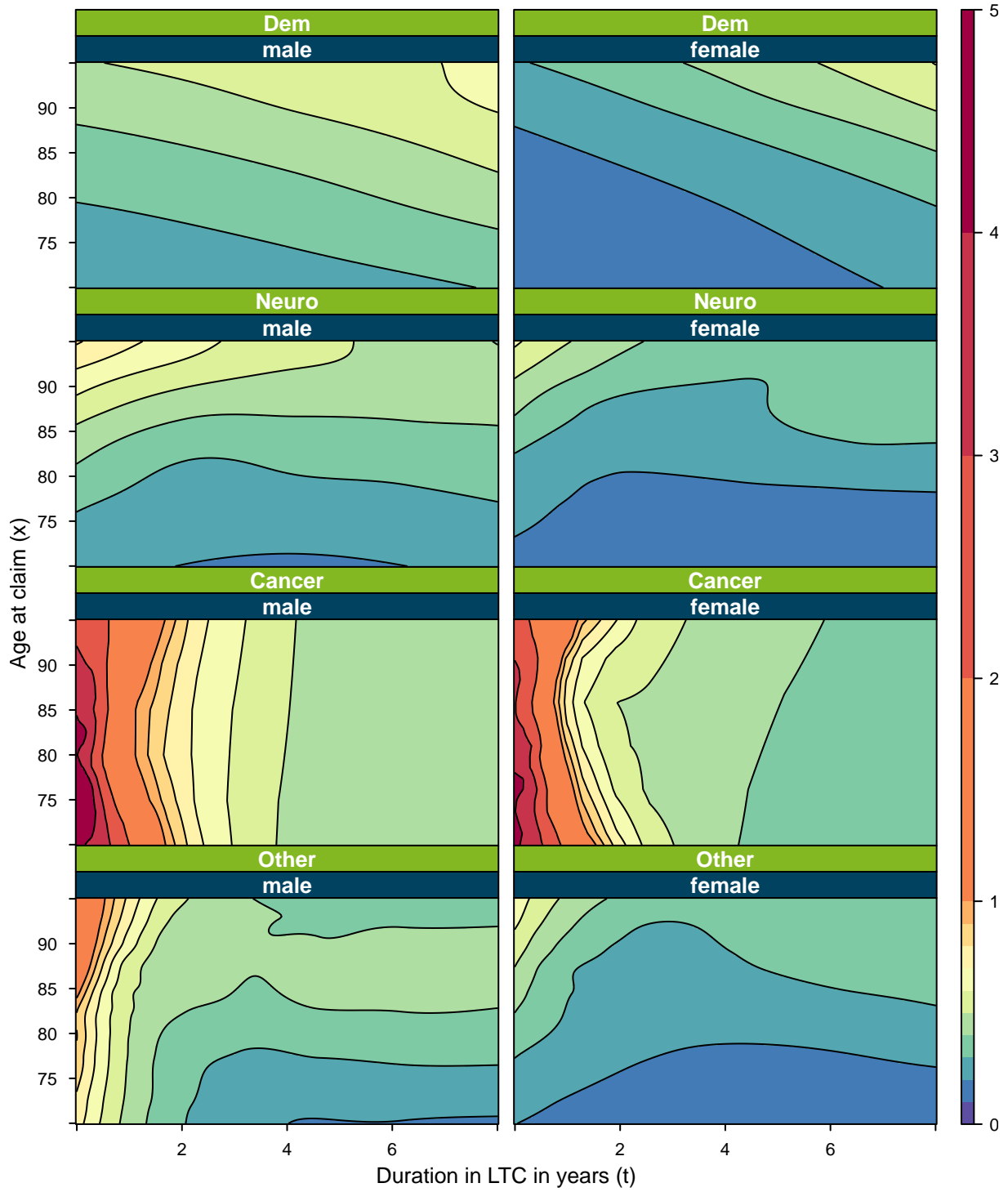
Figure 13: Cause-specific intensity of mortality in LTC obtained using local likelihood with optimal smoothing parameters.
