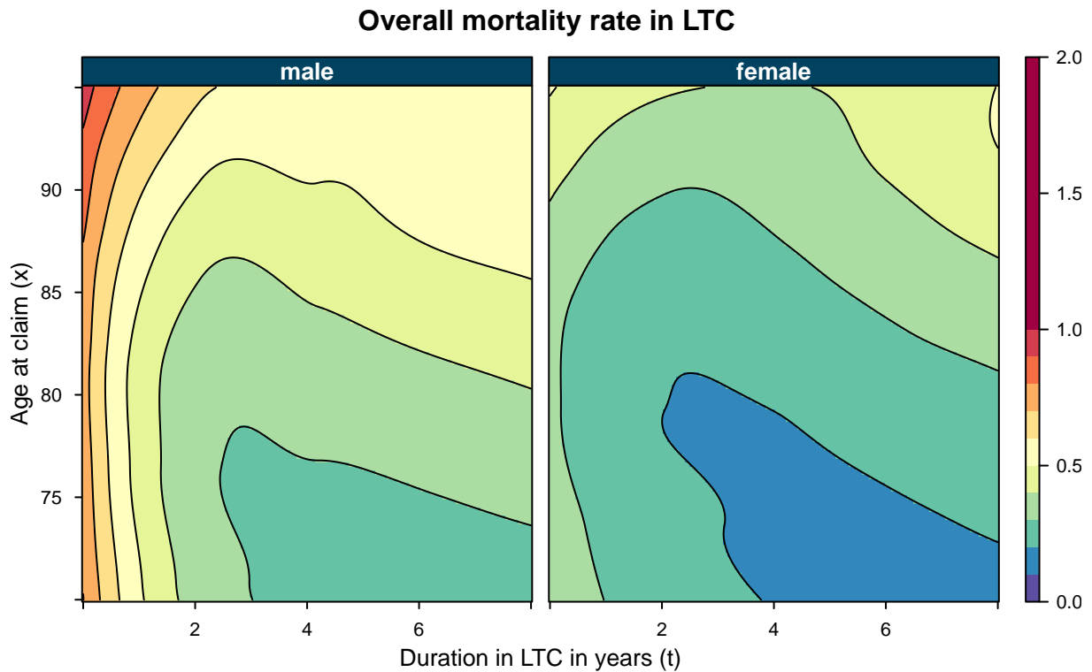
Figure 10: Intensity of mortality in LTC obtained using local likelihood with optimal smoothing parameters.
