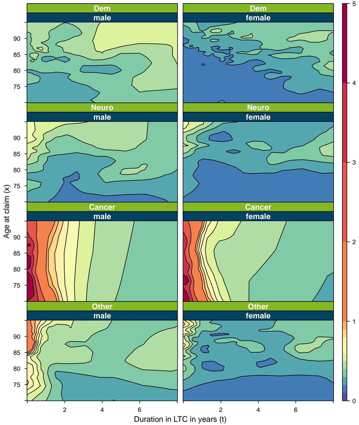
Figure 12: Cause-specific intensity of mortality in LTC obtained by using constant local fitting and distance to the 100-th nearest neighbours as bandwidth.
