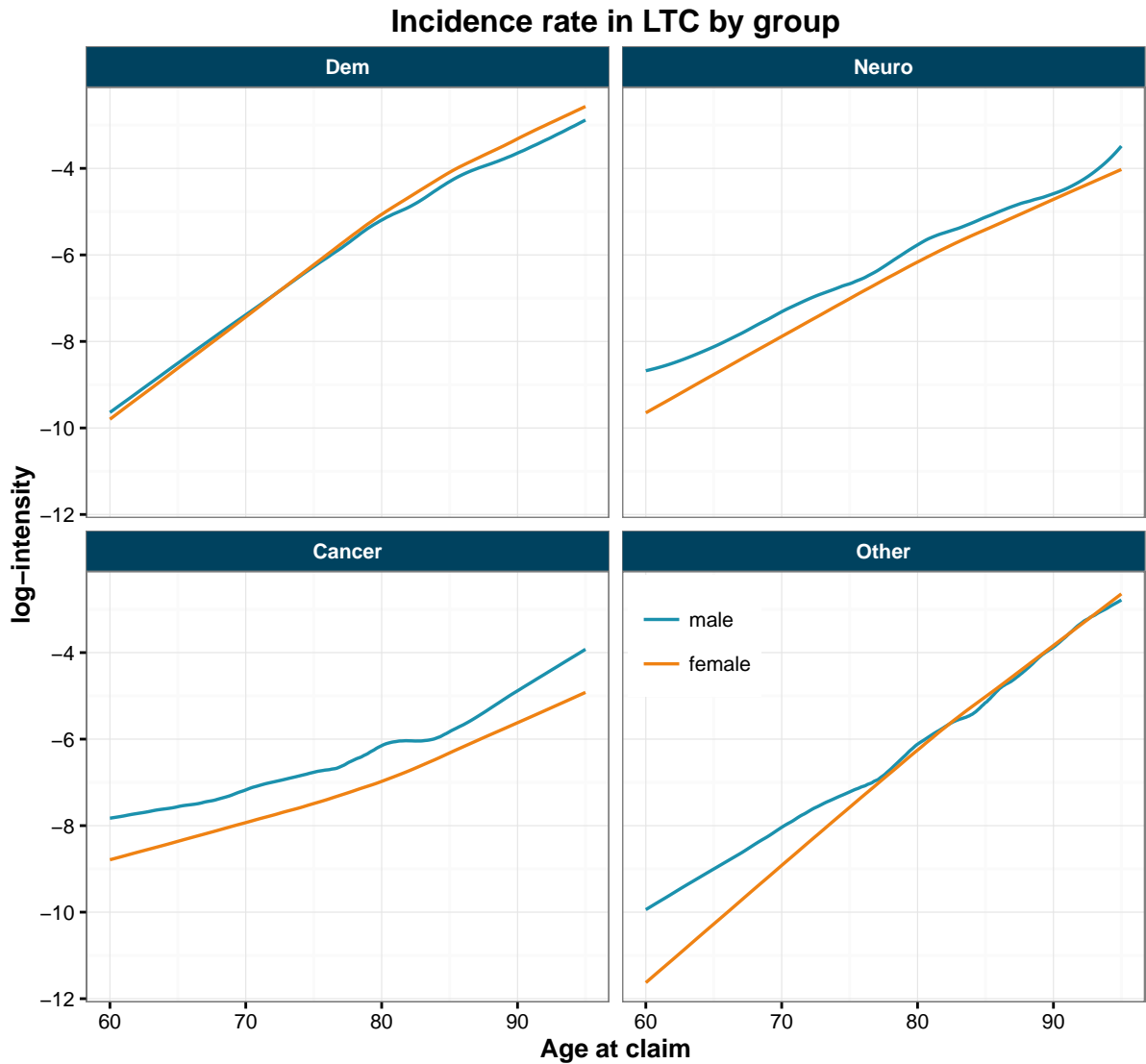
Figure 7: Intensity of incidence in LTC by group, estimated using local likelihood: logarithmic scale.
