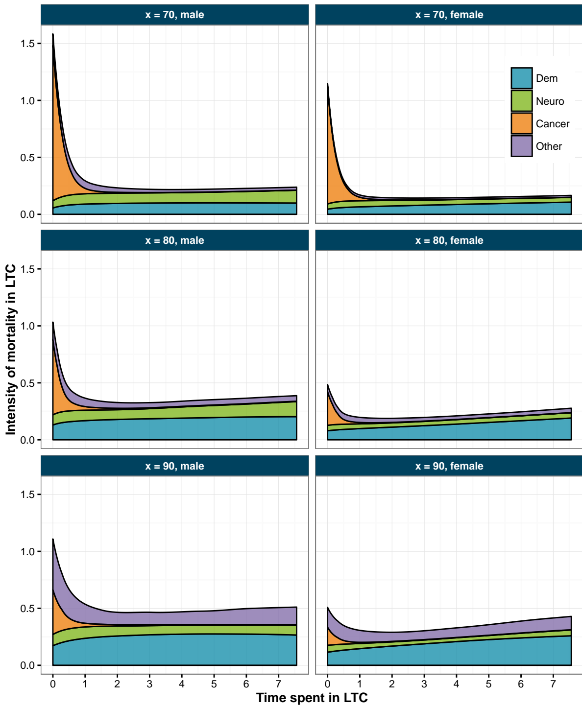
Figure 21: Contribution of pathologies to overall mortality in LTC.
