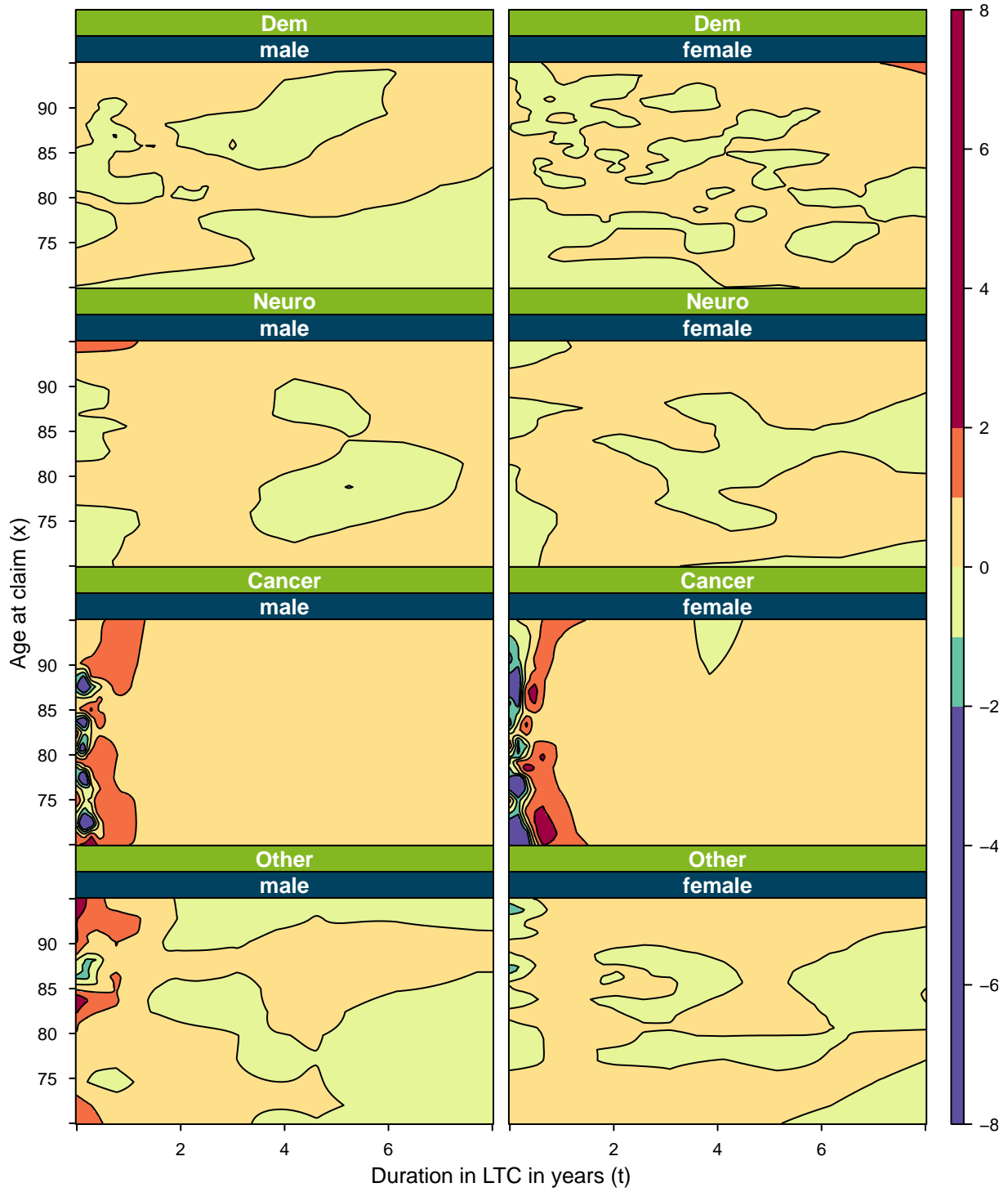
Figure 14: Pearson residuals associated with mortality in LTC by group.
