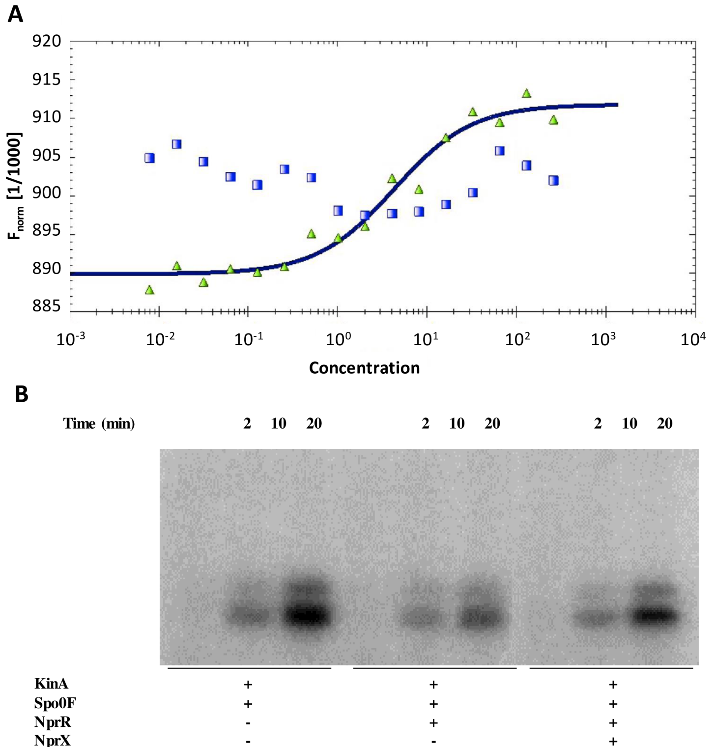
Fig 3. The sporulation inhibitor activity of NprR relies on Spo0F dephosphorylation. (A) Microscale thermophoresis analysis of the NprR-Spo0F interaction. The normalized NprR fluorescence F_{norm} , i.e. the “hot” fluorescence divided by the “cold” fluorescence, is plotted on a linear y-axis in per mil (%) against the total concentration of Spo0F on a log10 x-axis. The measurements were performed by using 20% LED power and 40% IR-laser power, in the presence (green triangles) and absence (blue squares) of NprX. (B) In vitro dephosphorylation of Spo0F-P by NprR. Purified B. subtilis Spo0F proteins (5.4 \mu M) was phosphorylated in a reaction containing B. subtilis KinA (0.1 \mu M) and [ \gamma - ^{32} P]-ATP. Purified NprR protein and synthetic NprX-8 peptide (SSKPDIVG) were added at 10 \mu M and 57 \mu M final concentration, respectively. Time course experiments were carried out and aliquots withdrawn at the indicated time points.
