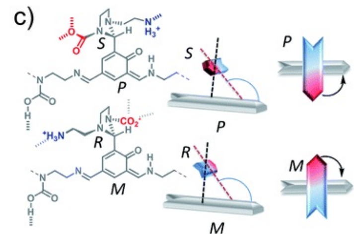
Fig. 3 Coupled configurational/conformational exploration of the junction between main and side chain around the connective center C_9 through (a) a short range ( \tau_{CP} = 500 \mu s ) DNP-enhanced ^1H - ^{13}C LG-CP HETCOR spectrum revealing spatial contacts. (b) Structural model with black arrows indicating correlations observed within the rigid backbone, and red arrows indicating observed correlations between flexible parts. This analysis leads to two possible enantiomeric monomeric units with opposite absolute coupled configuration/conformation on the C_9 center (c).
