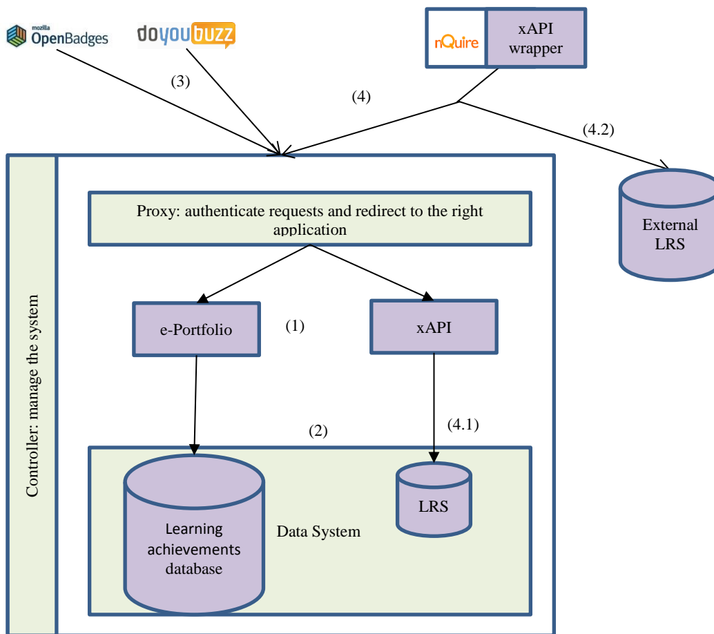
Figure 1. Prototype architecture
