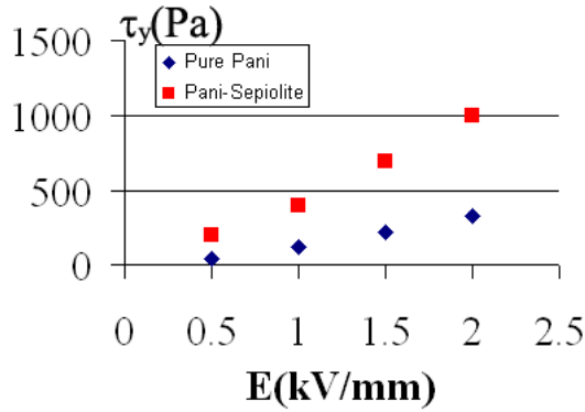
Figure 8. Yield stress versus electric field for a volume fraction \Phi=10\%
