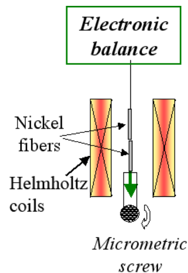
Figure 5. Schematic view of the device to measure rupture forces between fibers
