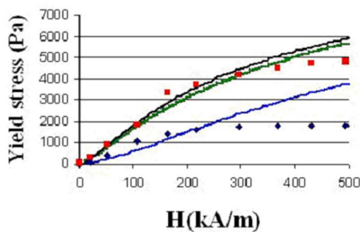
Figure 3. Yield stress versus magnetic field for a volume fraction \Phi=0.05 . Theory for fibers ( \xi=0.4, \Phi_a=0.5 ) ; theory for fibers ( \xi=0., \Phi_a=0.64 ); theory for spheres: ( \xi=0., \Phi_a=0.64 ); experiments for fibers; \blacklozenge \blacklozenge experiments for spheres experiments for cobalt fibers; \blacklozenge experiments for cobalt spheres
