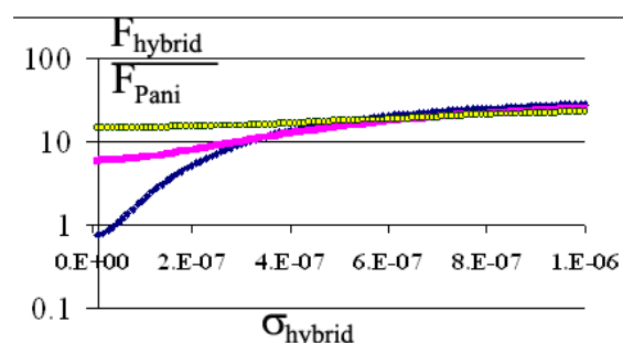
Figure 10. Ratio of the interparticle force (Eq.(14)) between hybrid particles to the one between pure PANi particles versus the conductivity of the hybrid particle for three values of permittivity: \epsilon_{\text{hybrid}}=137 ; \epsilon_{\text{hybrid}}=548 ; \epsilon_{\text{hybrid}}=1370
