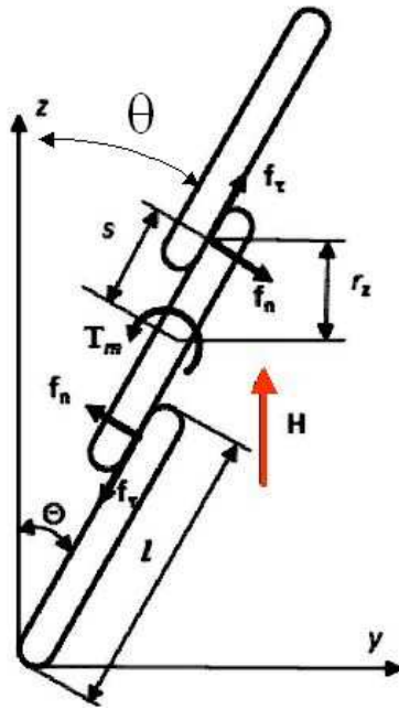
Figure 1. Schematic representation of contact forces between fibers
