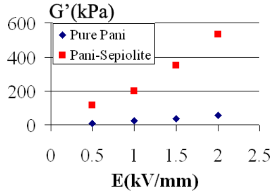
Figure 9. Shear modulus versus rms amplitude of the electric field at a strain amplitude of 0.03% and angular frequency \omega=20 rad/s
