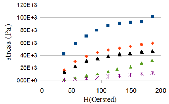
Figure 6. Rupture stress between fibers and chains of spheres with aspect ratio r=10 ■ ■ 2 cylinders with flat ends; ◆◆◆ cylinder with flat end and spherocylinder; ▲▲▲: 2 spherocylinders; ▲▲▲▲: 2 Chains of 10 spheres * * * : two spheres
