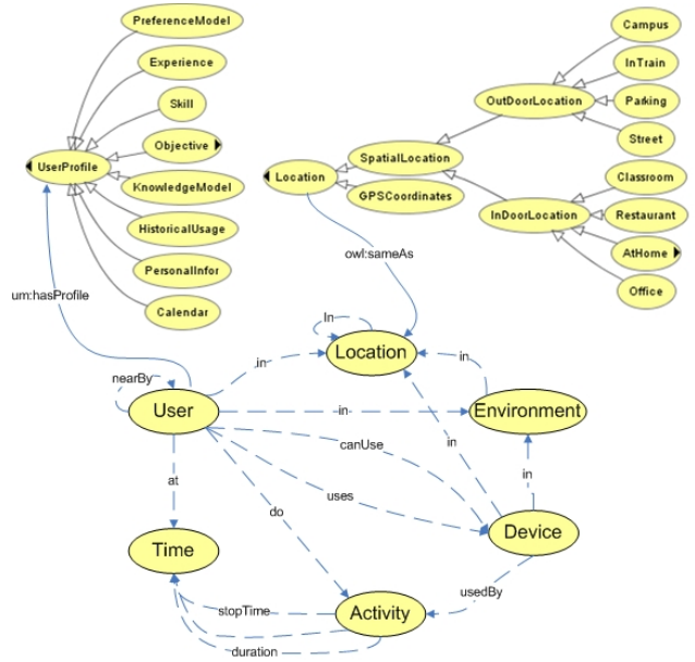
Figure 2. MUSE campus ontology (partial view)
