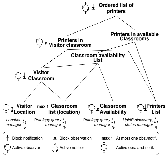
Figure 4. Context policy of "Nearest printers"
