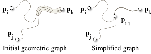
Figure 15: Two road paths (p_i, p_j) and (p_i, p_k) partially merging and resulting in a new Steiner point.
