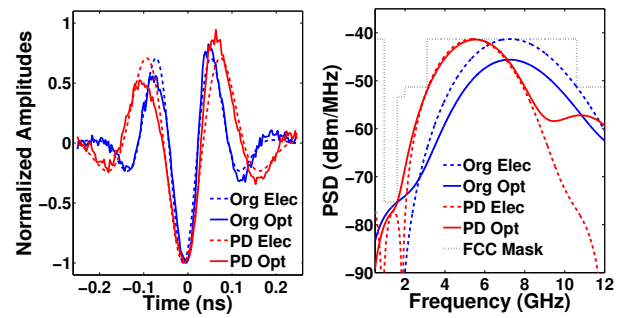
Fig. 7: Original (Org) and pre-distorted (PD) 6 th Gaussian, in electrical domain (Elec) and after SOA (Opt).
