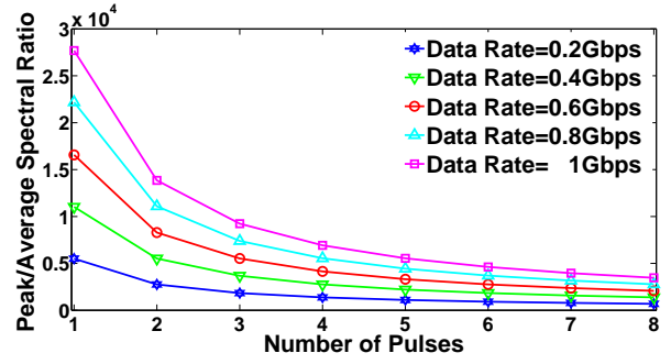
Fig. 3: The Peak-to-Average Spectral Ratio versus number of pulses used for PPM randomization, at different data rates.
