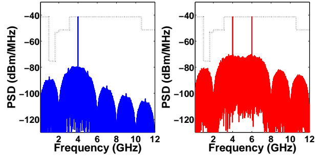
Fig. 4: Power Spectral Densities of 2Gbps standard OOK (left) and multi-waveform OOK based on 4 pulses (right).
