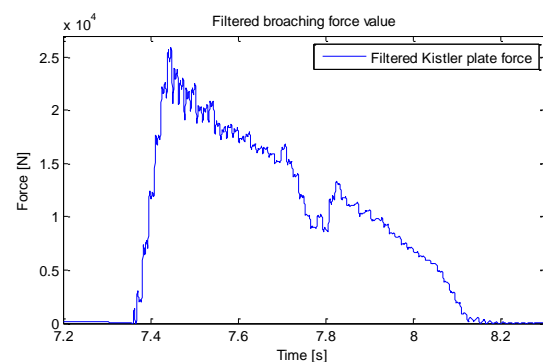
Figure 5. Filtered force signal (180Hz).
