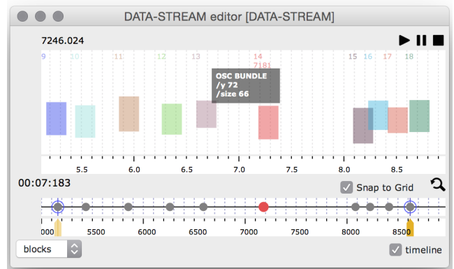
Figure 4. DATA-STREAM: a container and editor/renderer for timed data. In the patch at the top of the figure a sequence of dummy OSC-BUNDLES are generated and collected in the DATA-STREAM. Visualization parameters for these bundles in the editor (size, vertical alignment, colour) are either determined by searching for specific messages in the bundles (e.g. “/y”, “/size”), or just aleatory (e.g. colours).
