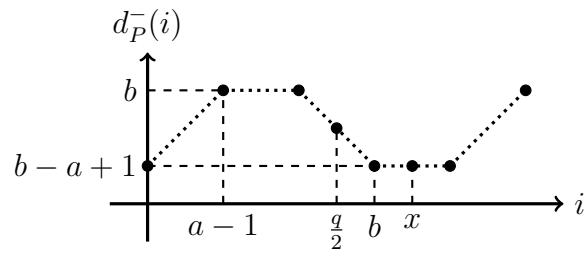
(b) a + b \neq q + 1 , q - b = b - a + 1 and a < q + 1 - b
