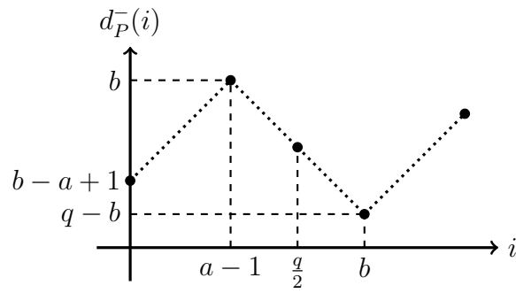
(b) a + b = q + 1 and q - b < b - a + 1
