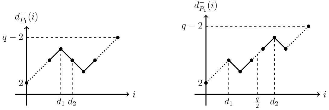
(a) \delta(P_1) = 2, \pi(P_1) = 0, d_2 - d_1 = 1 (b) \delta(P_1) = 2, \pi(P_1) = 0, d_2 - d_1 > 3
