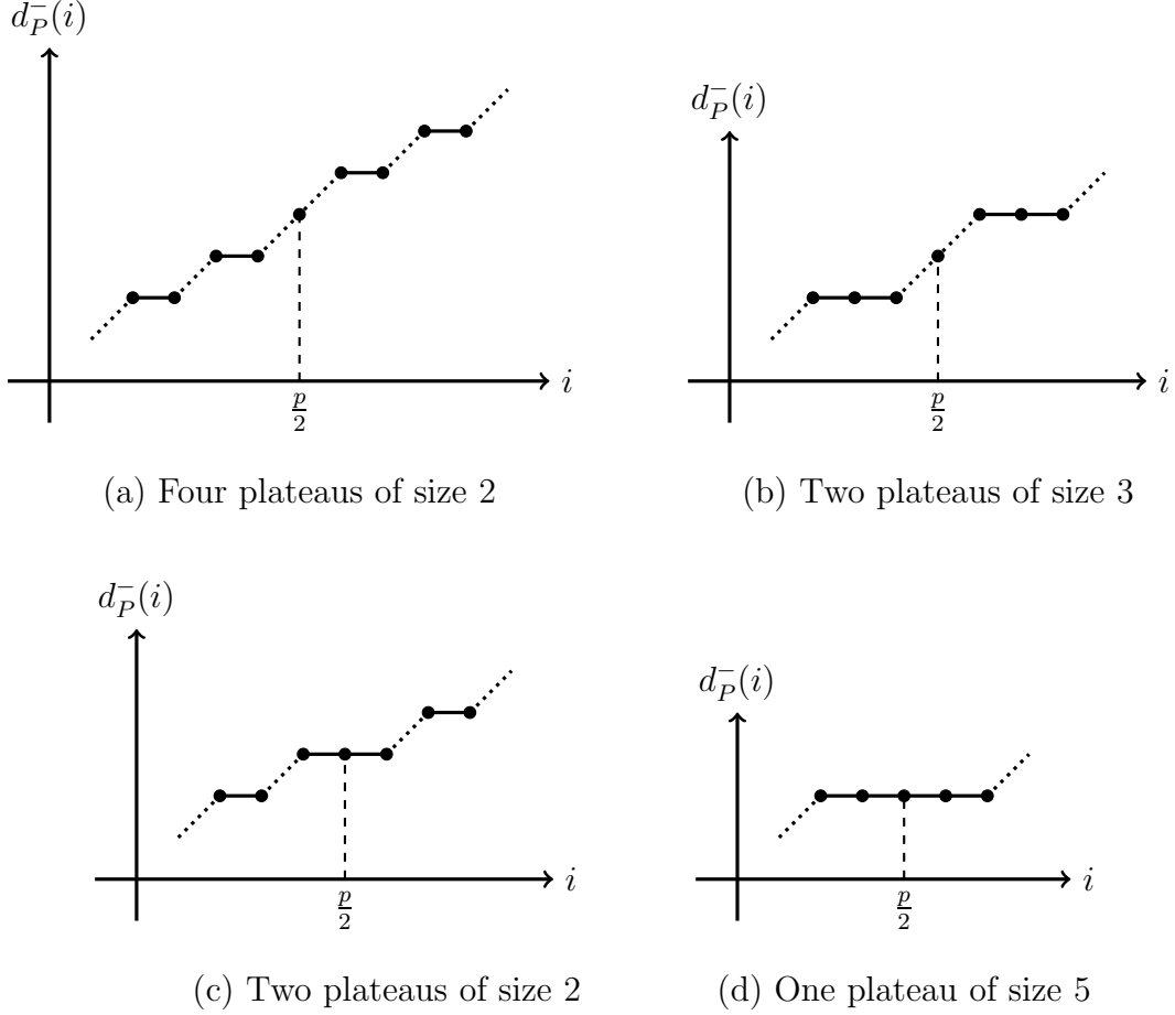
Figure 3: Indegree paths for the proof of Theorem 22 (Cont.)
