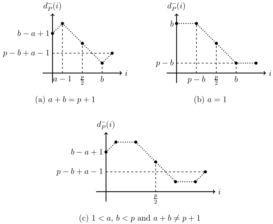
Figure 4: Indegree paths for the proof of Theorem 27, case b - a + 1 > \frac{p}{2}
