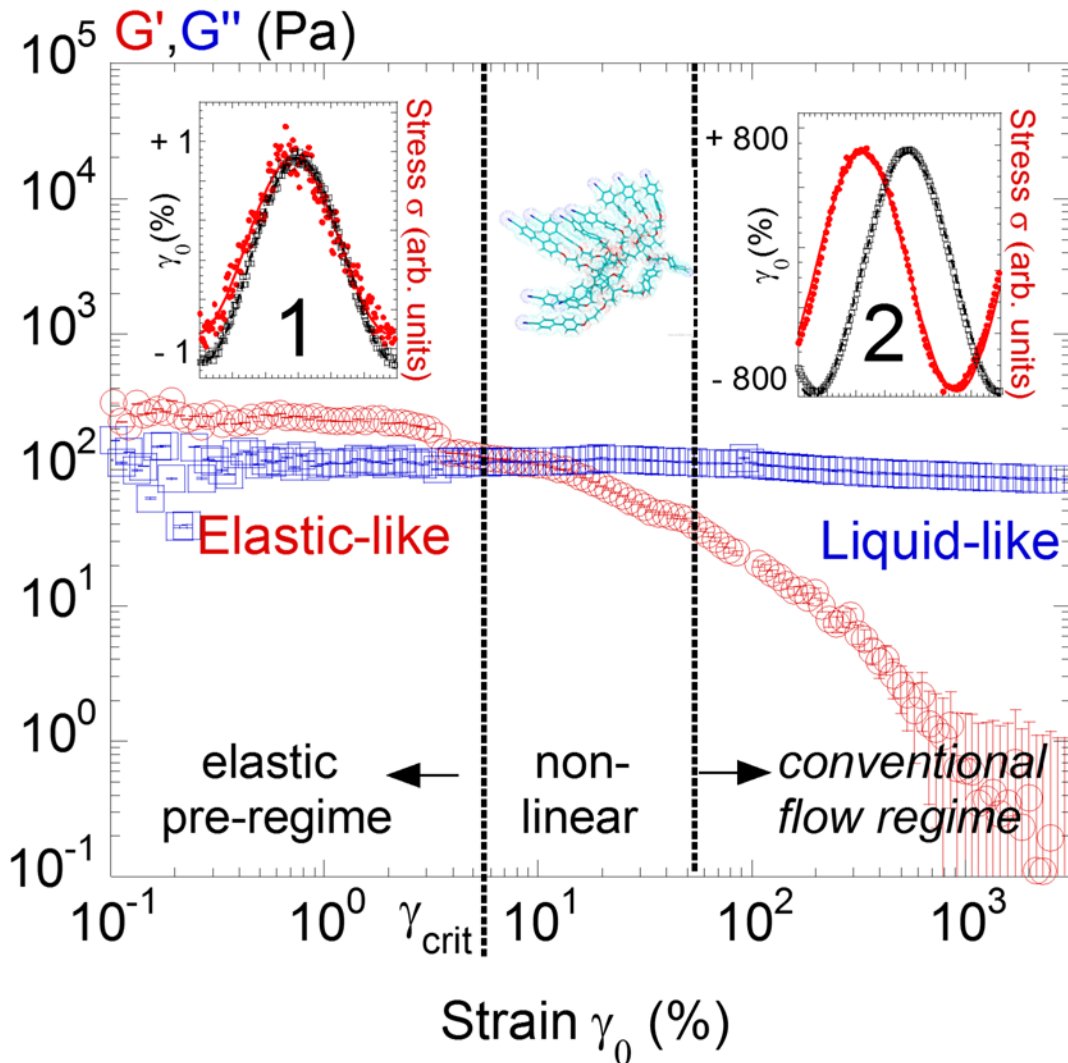
Fig 5. Identification of an elastic-like regime prior the Newtonian behavior in stress measurements: Stress dynamic moduli of LCF2 measured versus strain amplitude \gamma_0 at +25°C above the isotropic-smectic transition and for a gap thickness of 170 \mu m. Elastic modulus G' (red circles, \circ ) and viscous modulus G'' (blue squares, \square ) at a frequency of \omega = 0.5\text{rad s}^{-1} . The vertical dashed bar delimits the elastic regime (elastic-like behavior) at small strains \gamma_0 from the flow regime (liquid-like behavior) at large strains \gamma_0 . Insets: Raw periodic stress (red full dot: \bullet ) and strain (black hollow circles: \circ ) signals at small and large strain amplitudes ( \gamma_0 = 1.0\% and at \gamma_0 = 800\% respectively).
