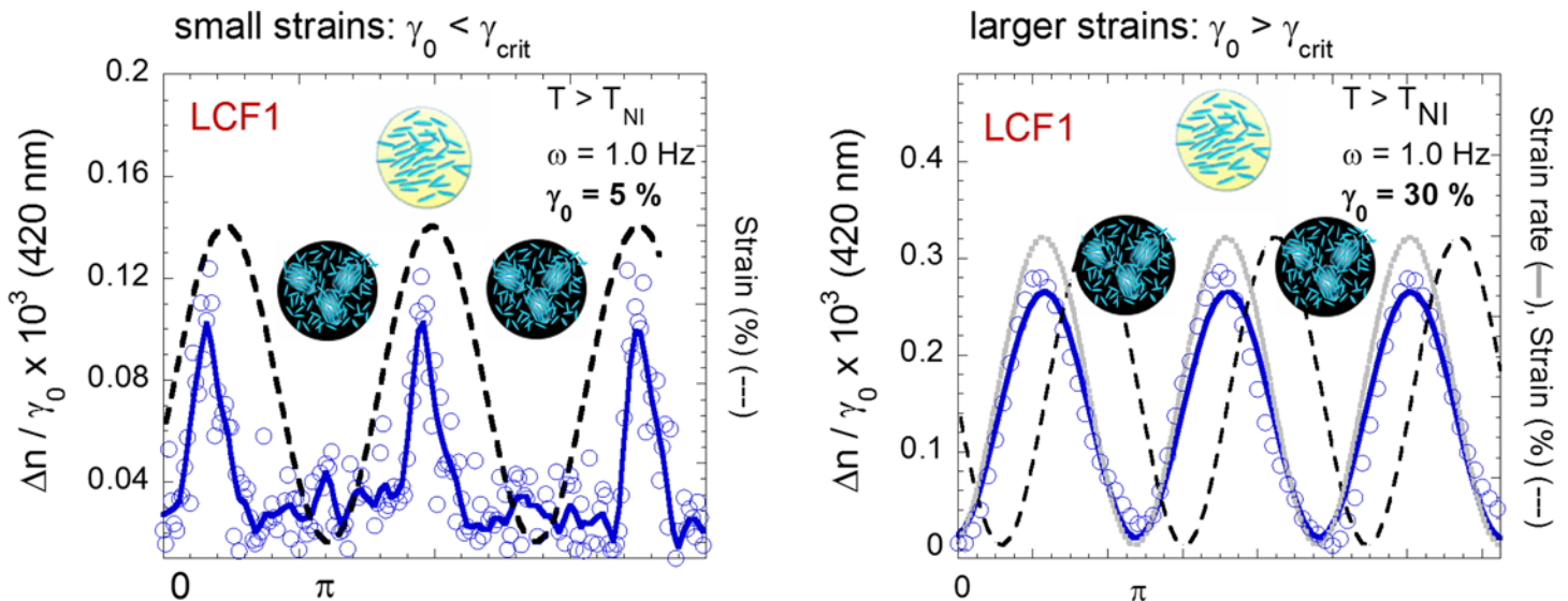
Fig 2. A mechanical oscillatory excitation at low frequency ( \omega = 1.0 Hz) orients the pretransitional fluctuations in the isotropic phase ( T - T_{NI} = +0.5^\circ\text{C} ) and creates a reversible and defect-free birefringent signal (sample: LCF1, blue circles \circ : sine model fit/smoothing of data points: continuous line, —). The birefringence values are normalized by the applied strain amplitude. (a) At small strain amplitude ( \gamma_0 = 5\% ), the optical signal is in phase with the strain (black dashed line, - - -). (b) At larger strain amplitudes (here \gamma_0 = 70\% ), the optical signal is synchronized with the strain-rate (continuous grey line, —).
