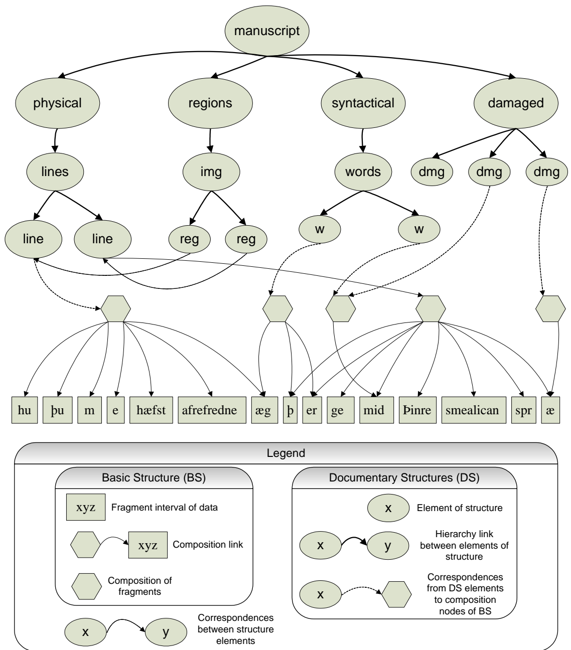
FIGURE 9 ILLUSTRATION OF THE MULTI-STRUCTURED DOCUMENT MODEL (MSDM)
