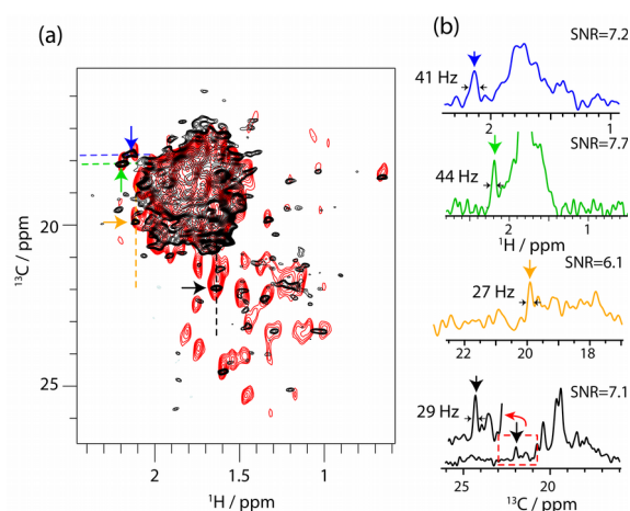
Fig. 3. Alanine methyl ssNMR spectra of Thermus thermophilus ribosome, obtained with 1.5 mg of deuterated, Ala- ^{13}\text{C}_3 labelled material. (a) 2D spectra obtained with INEPT-transfer (black, pulse sequence Figure S1E), obtained in a total time of 14 hours. The spectrum in red was obtained in 9 hours, using CP-transfers (sequence Figure S1A) with increased number of scans at the expense of resolution (see ESI for details). (b) 1D traces of the black spectrum along the ^1\text{H} and ^{13}\text{C} dimensions were extracted at the positions indicated with dashed lines, and the colours of the traces correspond to the colours of the arrows.
