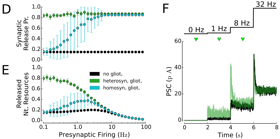
Figure 4: Gliotransmitter-mediated modulation of synaptic frequency response.
