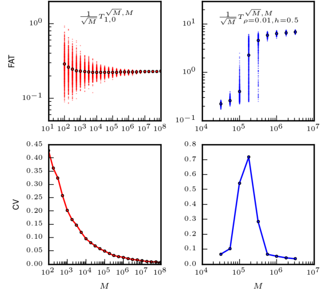
FIG. 8: First Assembly Time T_{1,0}^{\sqrt{M},M} (top left) and Generalized First Assembly Time T_{\rho,h}^{\sqrt{M},M} (top right) for the rescaled SBD and large maximal cluster size of order N = \sqrt{M} (section IIID 2) as a function of the total mass M (in log-log scale). Kinetics rates are p(x) \equiv 5 and q(x) = x . Both the FAT and the GFAT are divided by \sqrt{M} to verify the scaling in Eq. (34). Finally, the panels in bottom left and right represent the Coefficient of Variation (CV) as a function of the total mass M corresponding to the realizations of the upper panels.
