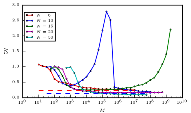
FIG. 4: Coefficient of Variation (CV) for the First Assembly Time T_{1,0}^{N,M} as a function of the total mass M corresponding to the realizations of Fig 3. For N = 6, 10 we plot additionally horizontal dashed lines at the value predicted by the Weibull distribution, see Eq. (15).
