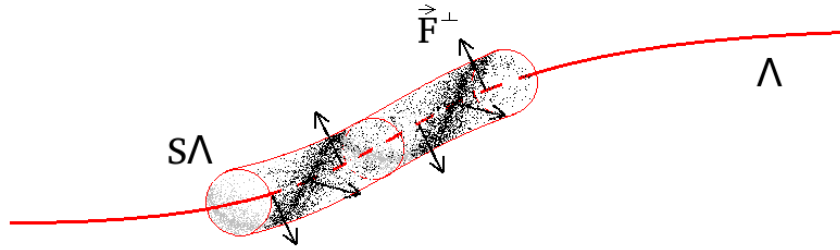
FIGURE 2. Above, we depict \Lambda encircled by its normal bundle in sphere S\Lambda (with fibers S_\sigma \Lambda = N_\sigma \Lambda / \mathbb{R}_+^* ). The mass concentration given by \nu is represented by the more or less strongly shadowed regions, and is directed by the normal force \vec{F}^\perp which is spinning around \Lambda in the example. Here, we took F(\sigma) = 1 and \nabla g(\sigma) = \mathbb{1} .
