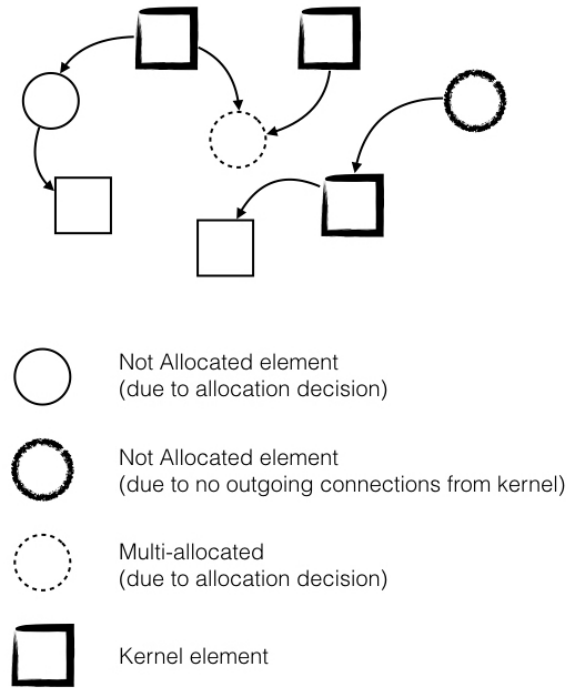
Figure 1. Example of allocation conflicts that may occur (each kernel element is associated to a different cluster)
