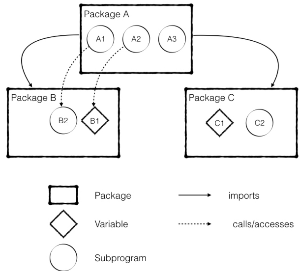
Figure 2. Example of a package imported but not used
