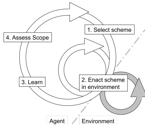
Figure 3: Algorithm procedure.
