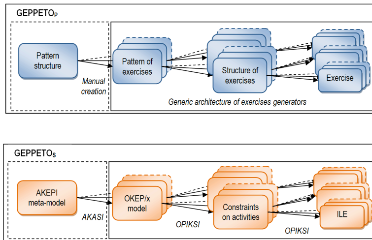
Fig. 2. Graphical representation of the GEPPETO P and GEPPETO S approach.
