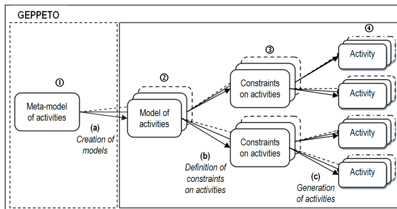
Fig. 1. Graphical representation of the GEPPETO approach.
