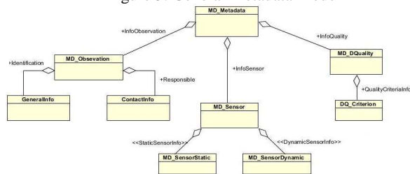
Figure 5: General Metadata Model
