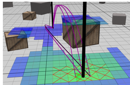
Figure 13: Potential targets: the color varies from green (best target) (score = 1) to blue (worst target) (score = 0). Crossed cells are the cells processed by our algorithm, in pink possible trajectories, in black the chosen one.
