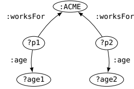
(b) Associated pattern graph
