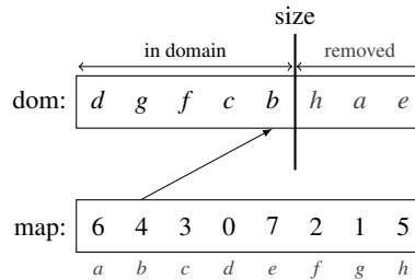
Fig. 5. Example representation of the domain \{b, c, d, f, g\} , such that \text{size} = 5 , when the initial domain is \{a, \dots, h\} . The \text{size} first values in dom belong to the domain; the last values are those which have been removed. The map array maps values to their position in dom. For example, value b has index 4 in the dom array. In such representation, only the size needs to be kept in the trail.
