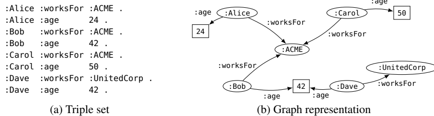
Fig. 1. RDF dataset example representing fictive employees.
