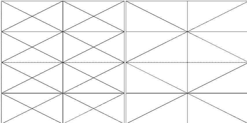
Figure 1. Start mesh for the P^1 case (left) and the P^2 case (right).
