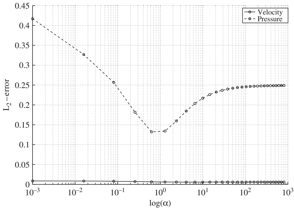
Figure 3. Effect of varying \alpha for the P^2 case.
