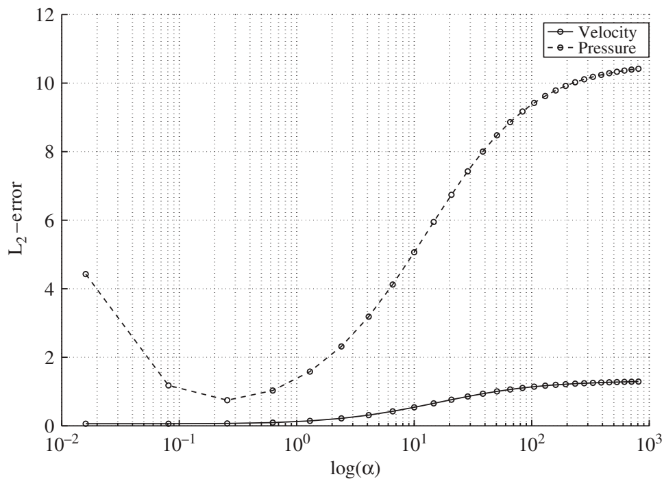
Figure 2. Effect of varying \alpha for the P^1 case.
